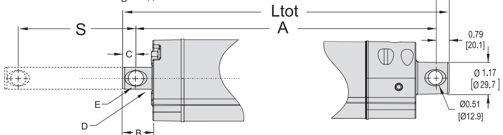
Type E front and rear adapter
