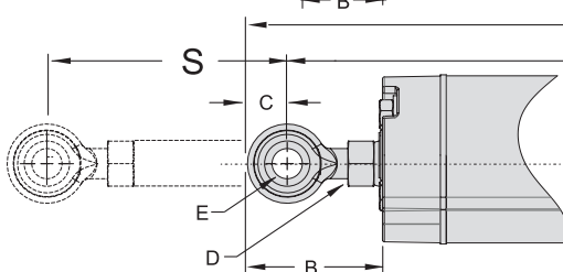
Type B front adapters
